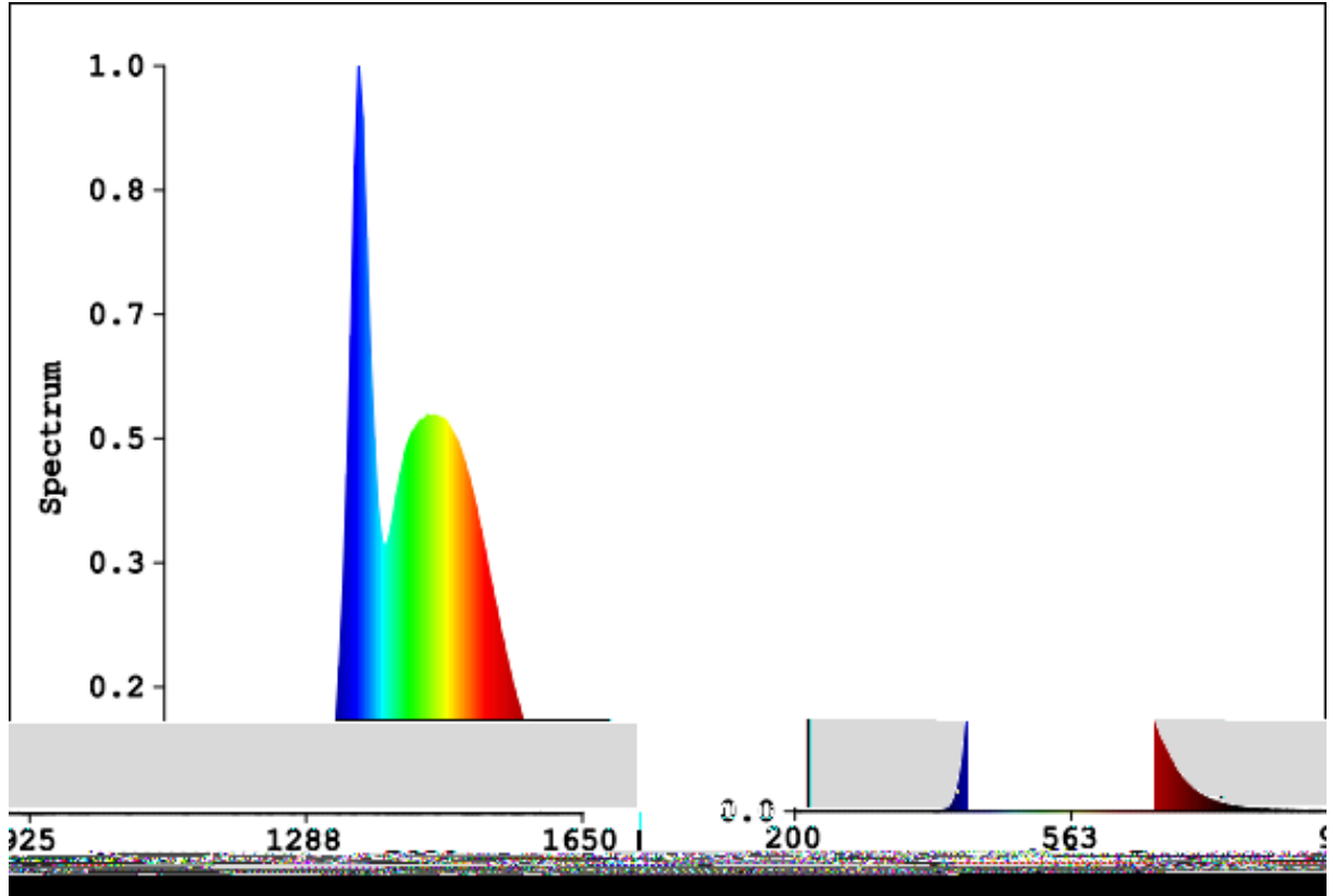
Spectral distribution
