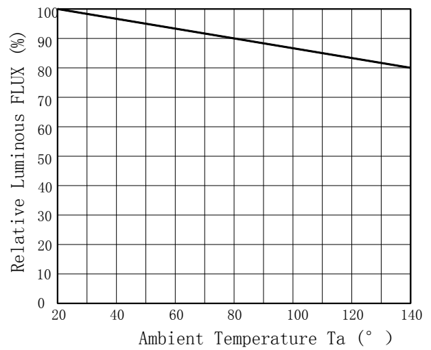
Relative Luminous Flux - Ta
